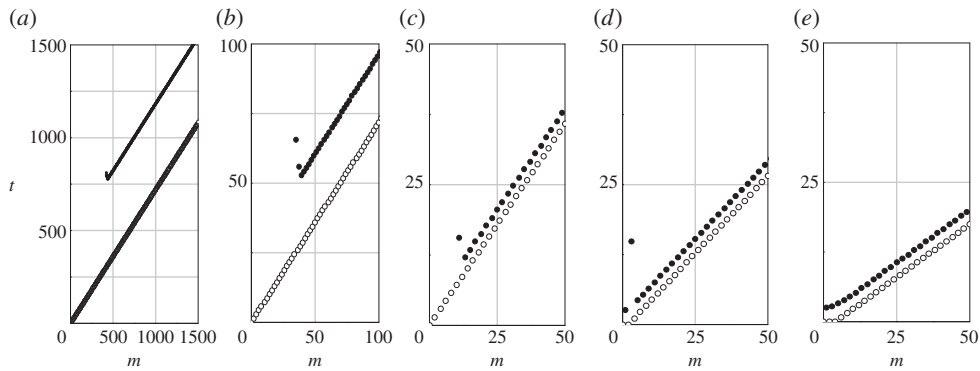
Figure 16. Results of the numerical simulations. The propagation of a partially bridged crack. The modes are presented where the initially compressed bonds break at an energy-dependent distance behind the crack front. In the numerically examined transient problem, the odd-bond breakage begins at a distance from the starting point of the dynamic crack. The latter distance as well as the former vanishes as the energy approaches the upper critical bound. In a general case of the steady-state regime, the length of the bridge crack zone is invariable. As can be seen in plot (c), there is a forward–backward splitting, the bonds break in the order 2m \rightarrow 2m - 3 \rightarrow 2m + 2 \rightarrow 2m - 1 \rightarrow \dots (a) \gamma = 0.946 (b) \gamma = 0.947 (c) \gamma = 0.948 (d) \gamma = 0.990 (e) \gamma = 0.999 .
