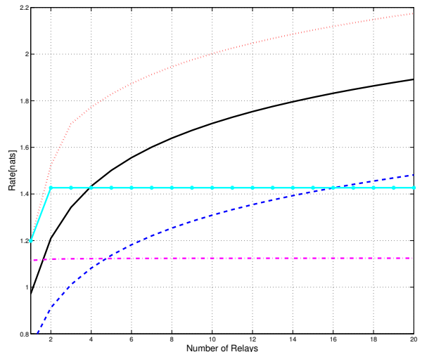
(b) \rho = 0.5 , \text{SNR}_{\text{BC}} = 150 , \text{SNR}_{\text{MAC}} = 10
