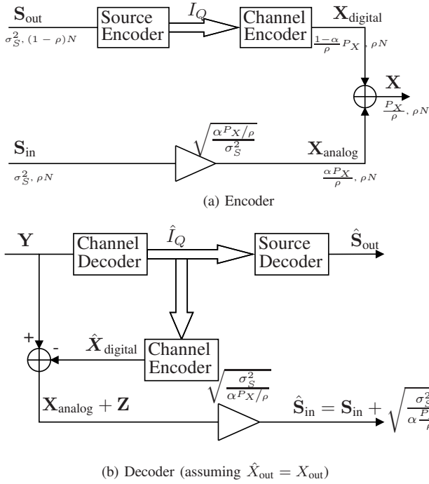
Fig. 7: HDA Scheme for BW Compression.
