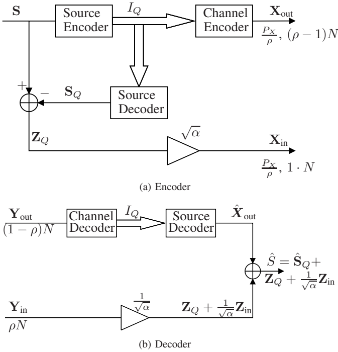
Fig. 6: HDA Scheme for BW Expansion
