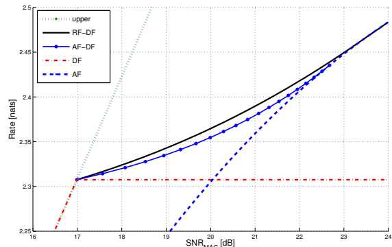
Fig. 9: Time-sharing for the equal-BW case. M = 2 , \text{SNR}_{\text{BC}} = 100 .
