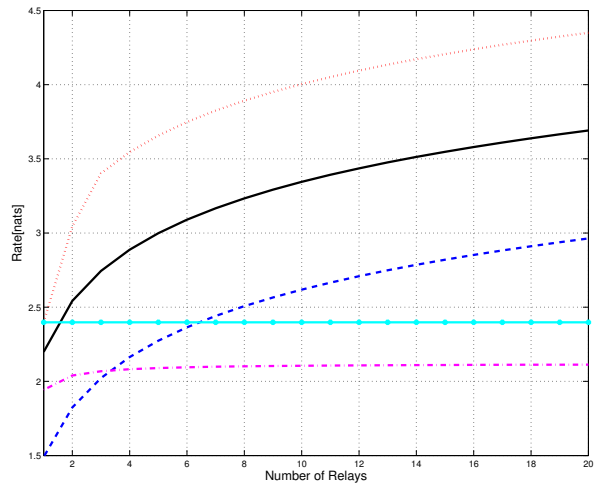
(a) \rho = 2 , \text{SNR}_{\text{BC}} = 20 , \text{SNR}_{\text{MAC}} = 300
