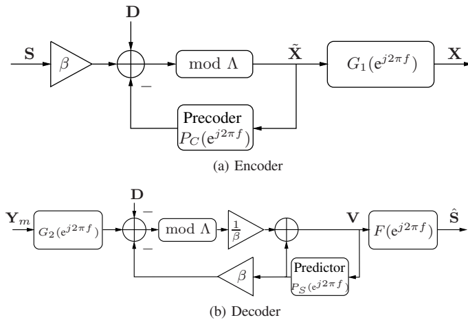
Fig. 10: Analog Matching encoder and decoder for R&F
