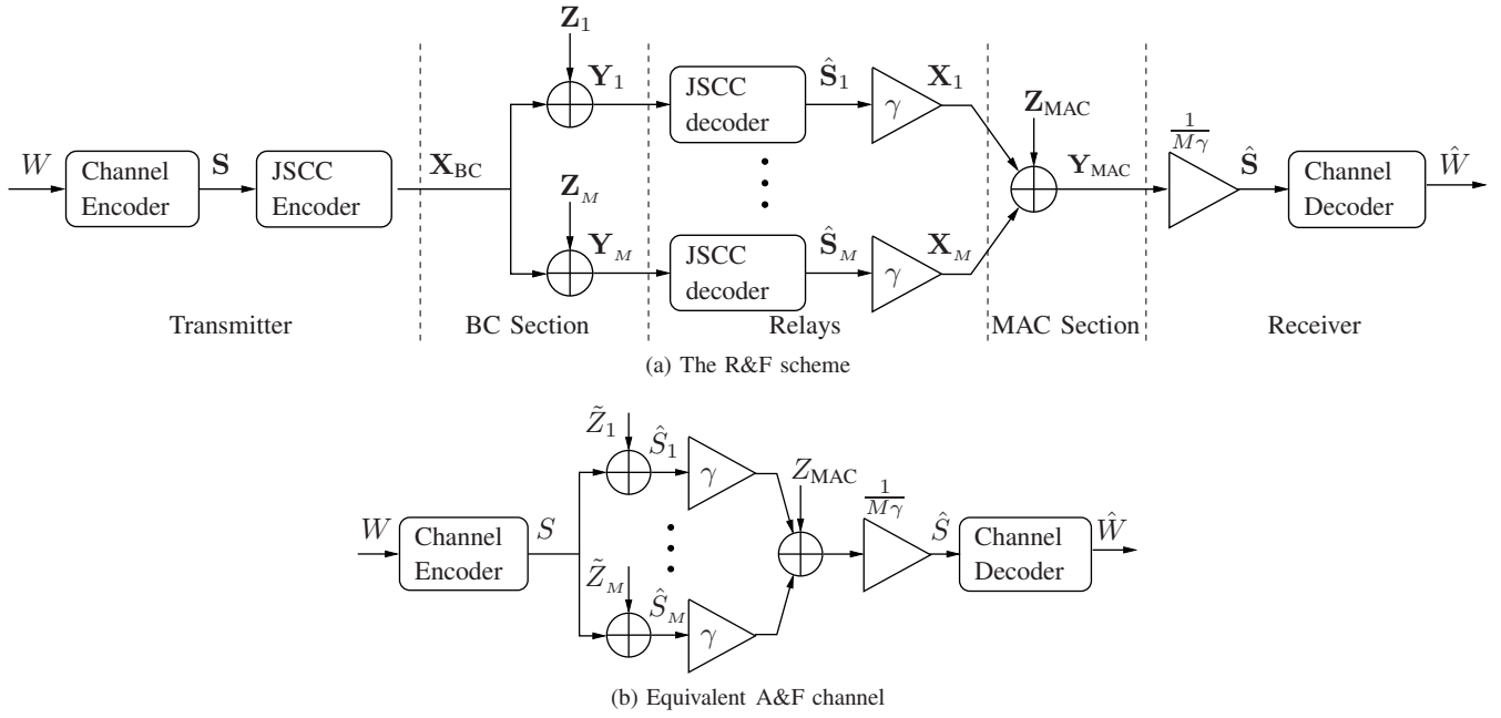
Fig. 5: The R&F Strategy for the parallel relay network.
