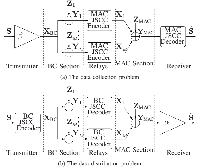
Fig. 4: Sensor network problems and the parallel relay network.
