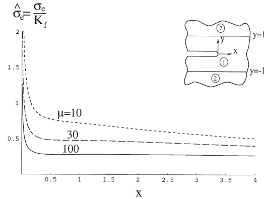
Fig. 3. Influence of the shear moduli ratio \mu = \mu_2/\mu_1 of the composite constituents on the stress distribution in front of the crack in the eigensolution for typical values \nu_1 = 0.35 and \nu_2 = 0.3 .
