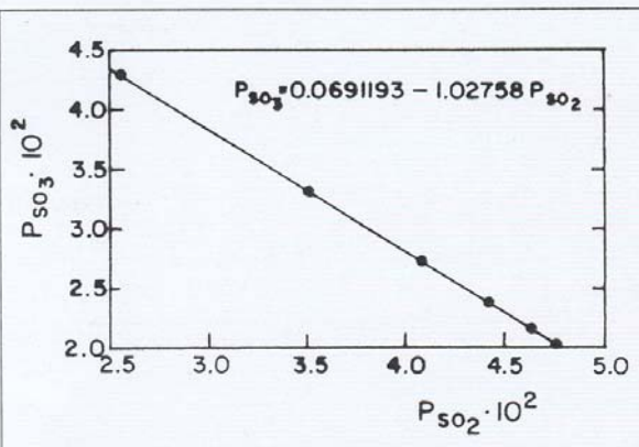
Figure 3. Linear dependency between p_{SO_3} and p_{SO_2} in the experiments.
