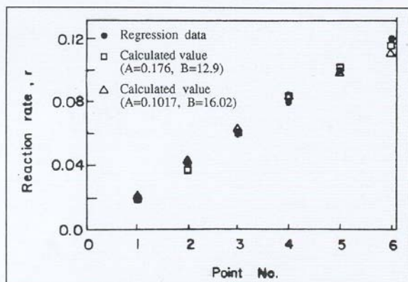
Figure 1. Experimental and calculated reaction rate, using Eq. (1) as rate expression
