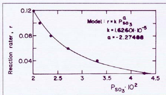
Figure 2. Calculated curve and experimental data versus P_{SO_3} with power-law expression
