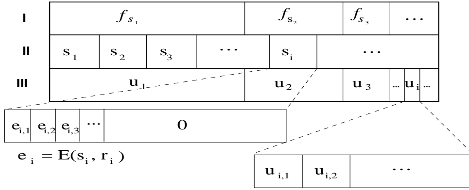
Figure 1: Construction for Theorem 1.1
