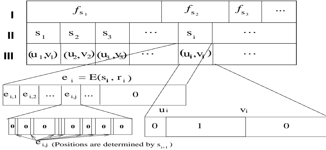
Figure 2: The General Construction with the Query Equalizer (analyzed in Item 2 of Theorem 1.6)
