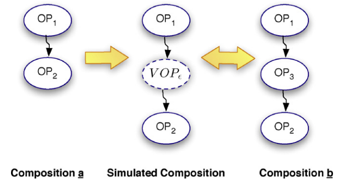
Fig. 5. An example of applying the behavioral pattern: composition a is matched with composition b by simulating b with a . If such a simulation exists, then the similarity is defined by its construction cost.
