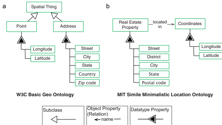
Fig. 1. Location specification using two different ontologies. Logic-based approaches would return the correct result when the service is specified using ontology (a), but would fail to do so when the service is specified using ontology (b).
