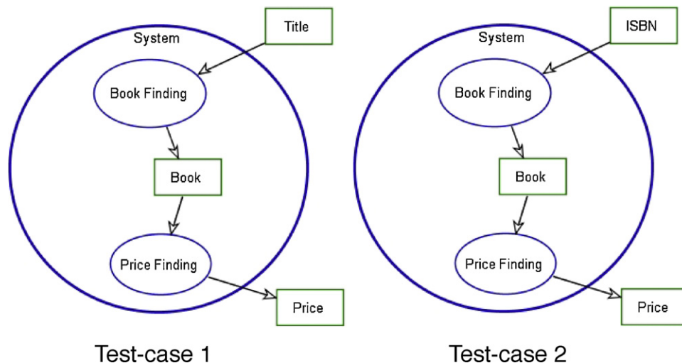
Fig. 6. An example of two test cases on the same query: “Find the price of a book according to the book’s title”.
