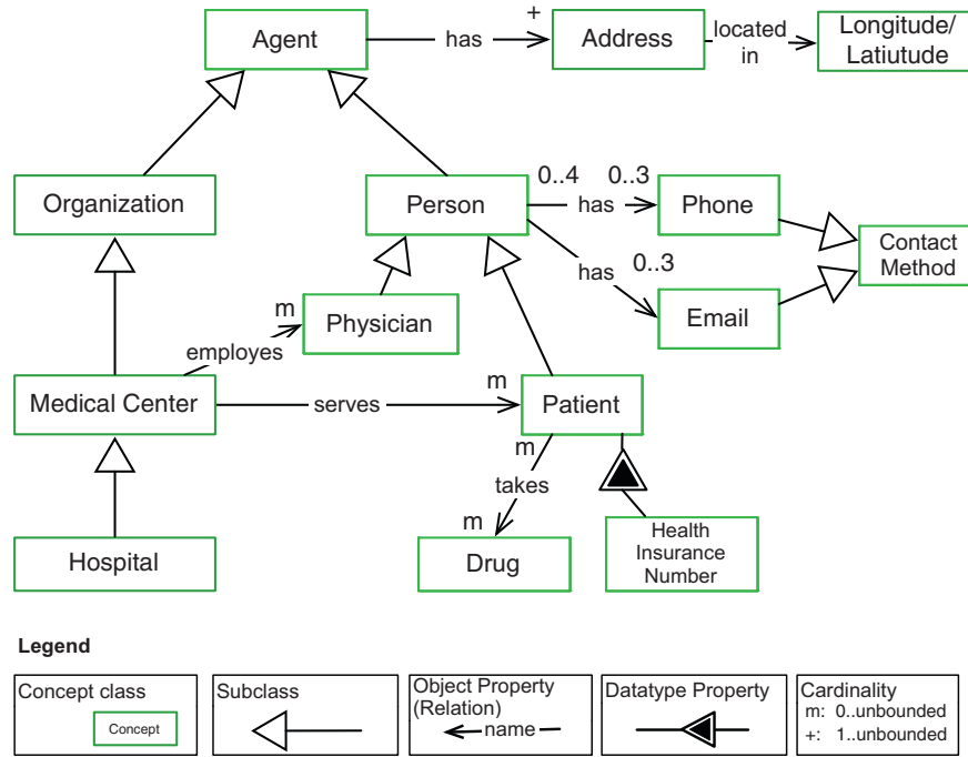
Fig. 3. An example of a healthcare ontology, including concepts, subclass relations, object properties, and datatype relations.
