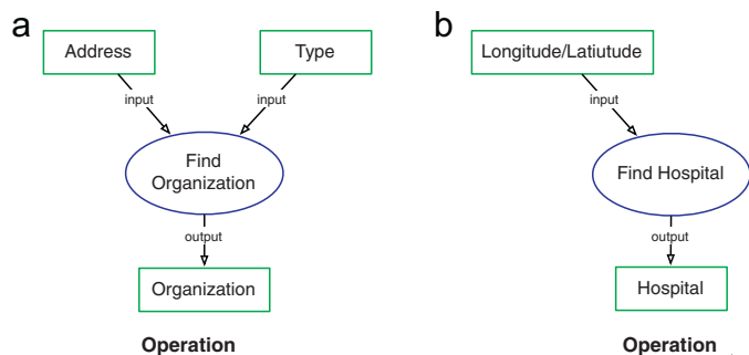
Fig. 2. Two operations which can possibly answer the query “Find a service that accepts an address and returns the closest hospital”. The “closest to” ontological relation is not displayed.
