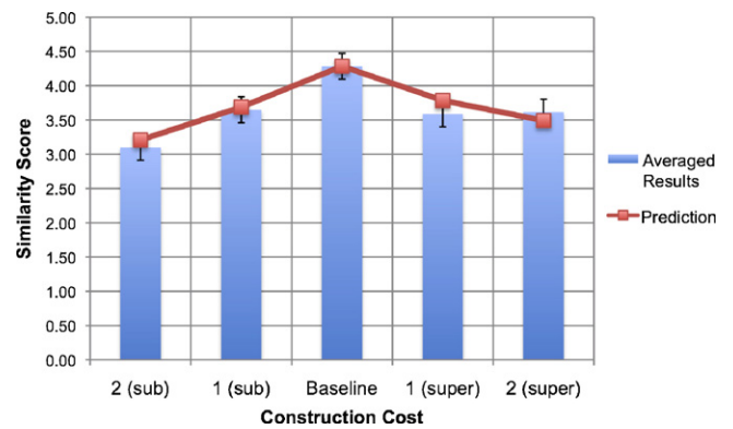
Fig. 7. Set-hierarchy pattern similarity assessment. The X-axis represents the cost construction, based on the set hierarchy distance. The Y-axis represents the similarity. The bars are the averaged results over all the test cases, and the line represents the prediction of our model.
