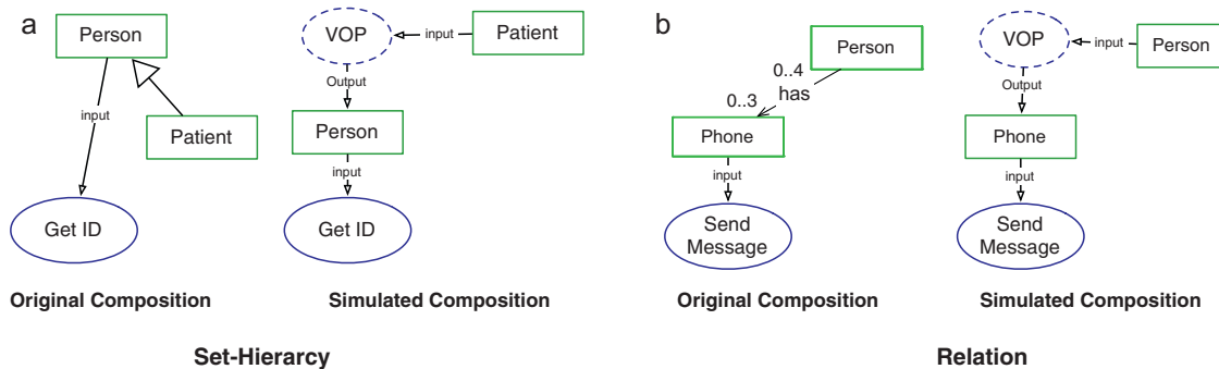
Fig. 4. Examples of applying the set-hierarchy and relation pattern.
