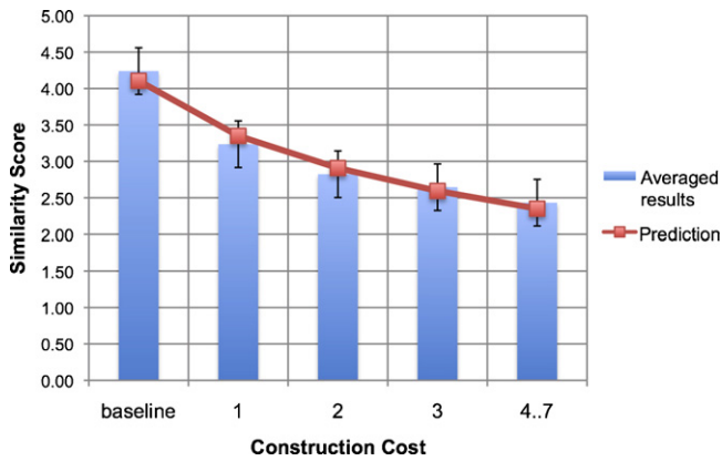
Fig. 8. Relation pattern similarity assessment. The X-axis represents the cost-constructions, based on the set relation cardinality. The Y-axis represents the similarity. The bars are the averaged results over all the test cases and the line represents the prediction of our model.
