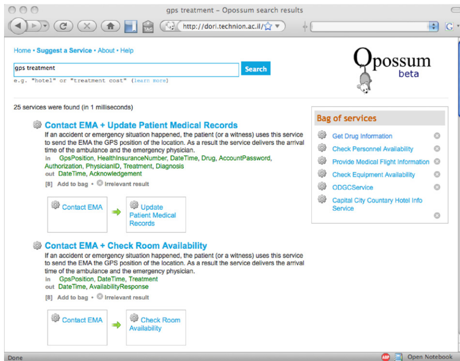
Fig. 11. Compositions ranked and retrieved by the OPOSSUM search engine. The search engine was updated with the semantic similarity patterns defined in this study.
