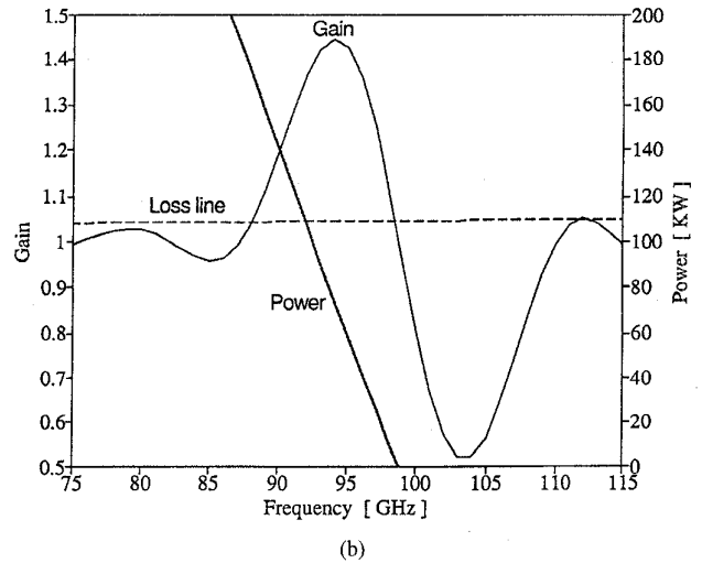
Fig. 5. Performance parameters of an EA-FEM: gain (solid curves), extracted power (heavy solid curves) and resonator ohmic losses (dotted curves). (a) Operating frequency near 35 GHz. (b) Operating frequency near 94 GHz.
