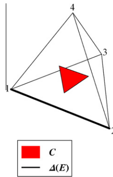
Fig. 2.1. The set of probability measures C for our leading example (see Example 2.1). Updating of C must result in a subset of \Delta(E) .
