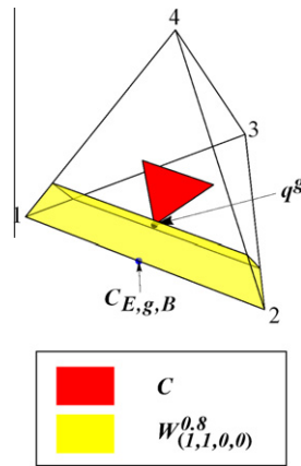
Fig. 3.3. Illustration of Algorithm 3.3 for computing the update rule U^{DC \cap R \text{Amax}} (see Example 3.3).
