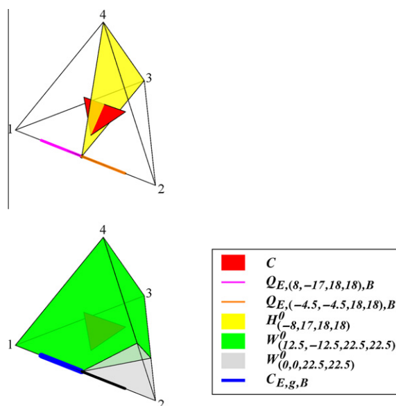
Fig. 3.2. Illustration of Algorithm 3.2 for computing the update rule U^{DC \cap \text{PFI} \max} (see Example 3.2).
