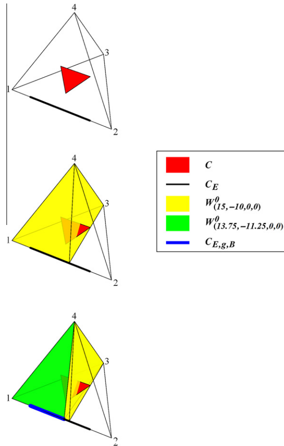
Fig. 3.1. Illustration of Algorithm 3.1 for computing the update rule U^{DCmax} (see Example 3.1).
