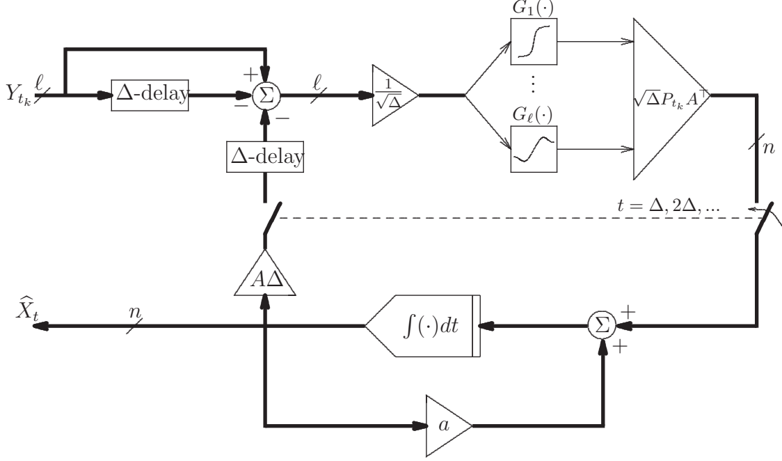
FIGURE 1. Block diagram of the proposed filter
