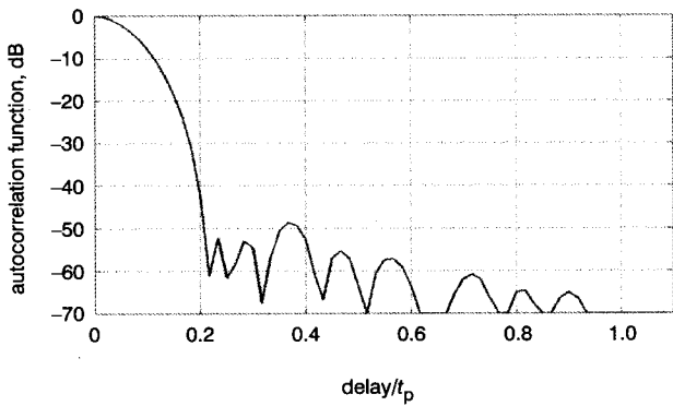
Fig. 16 Partial autocorrelation function of 120 pulses with the frequency steps shown in Fig. 14
