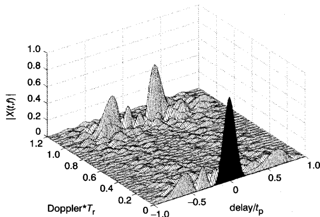
Fig. 17 Partial ambiguity function of the NLFM signal defined in Fig. 14
