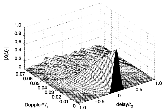
Fig. 18 Doppler zoom of data in Fig. 17
