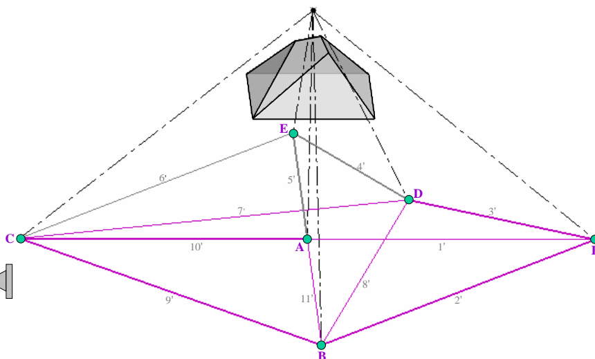
The reciprocal diagram=Maxwell Cremona diagram
