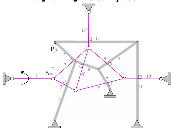
The duality between trusses and mechanisms (infi truss is dual to a locked mechanism)
