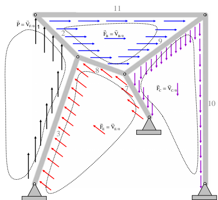
The original linkage in a locked position
