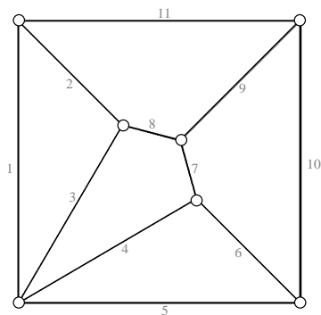
The original framework-determinate truss with a self stress
