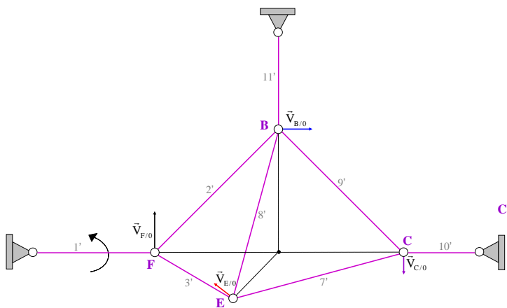
The truss underlying the diagram (not stable truss=infi truss)
