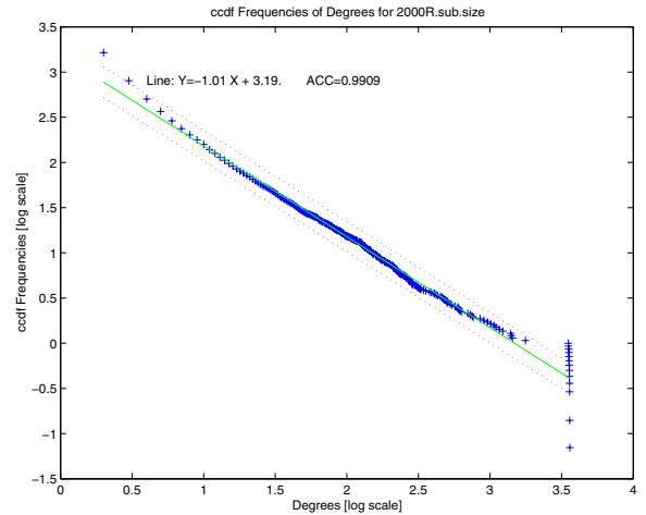
Fig. 3. Sub-tree size CCDF distribution, for a 2000 node tree cut from topology a_0 = 6, a = 2, p = 0.1, q = 0 .
