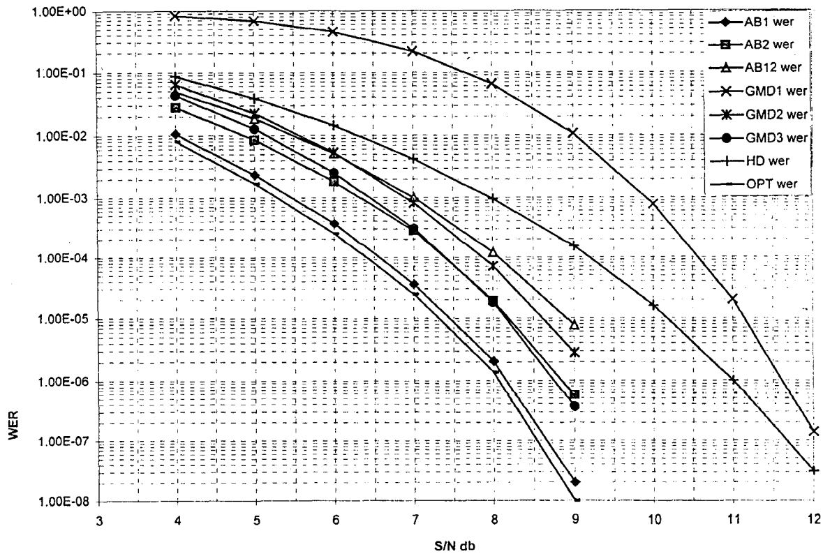
Figure 2: (8,4,4) code over GF(4)
