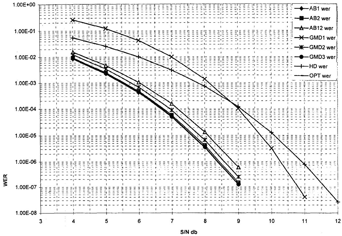
Figure 1: Binary (8,4,4) extended Hamming code
