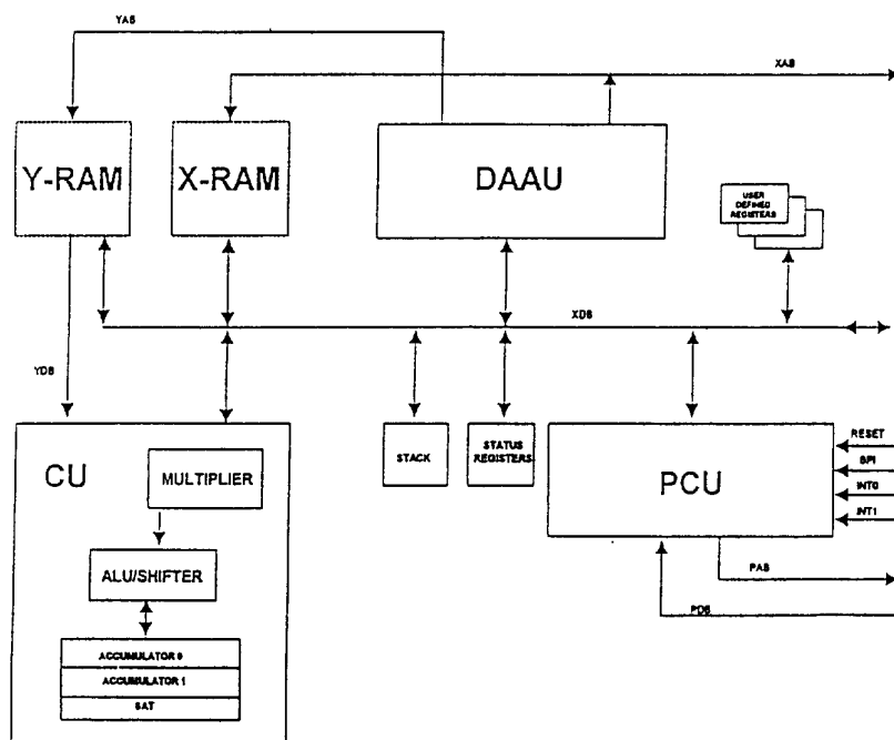
Figure 1. PINE Block Diagram
