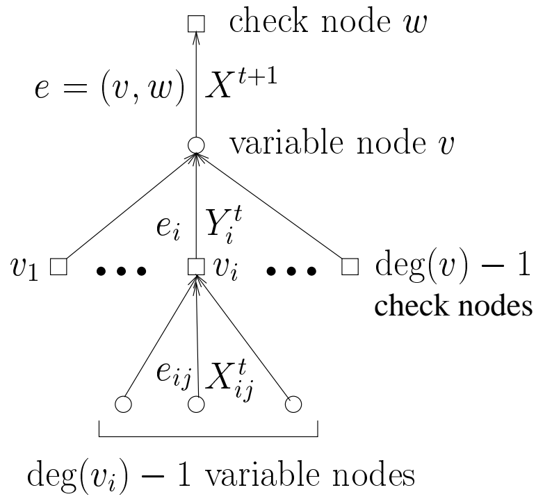
Figure 1: A depth two tree spanned from e = (v, w) .
