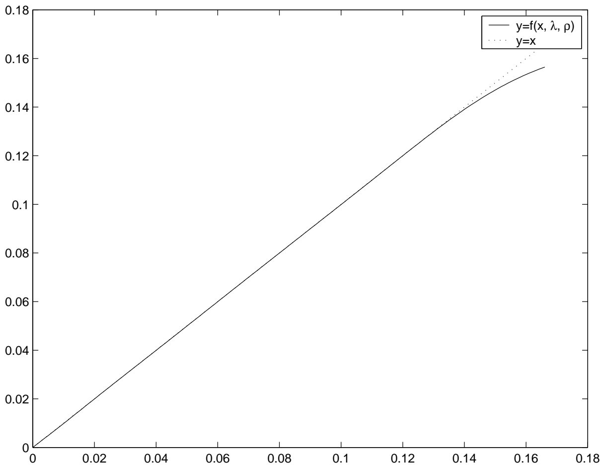
Figure 3: A plot of f(x, \lambda, \rho) for rate 1/2 irregular LDPC code. The crossover parameter is p = 0.092 .
