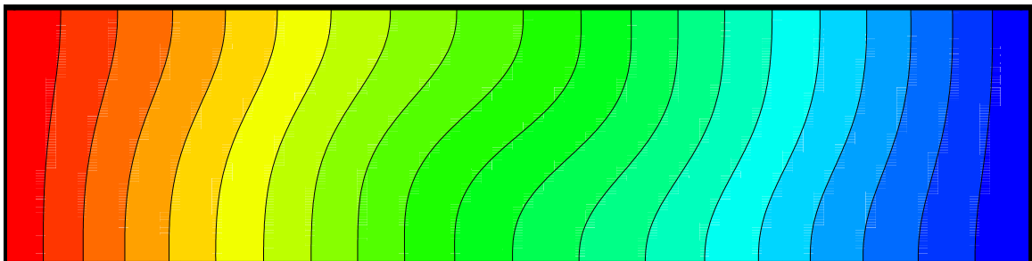
isotherms
