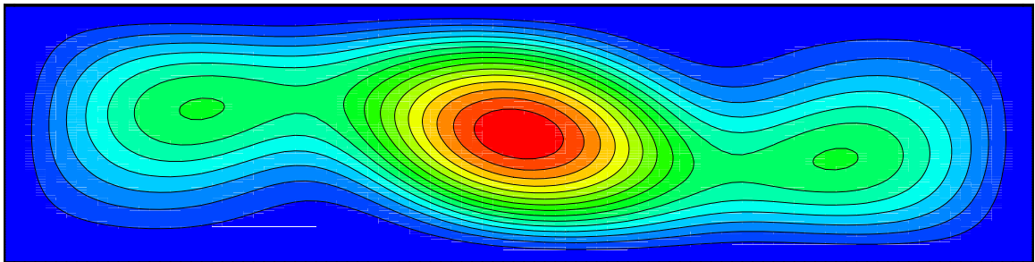
streamlines
