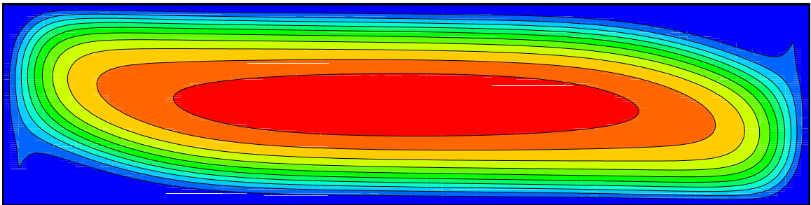
streamlines
